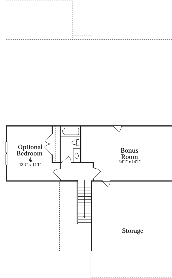
Opt. Second Floor Plan With Bonus Room
